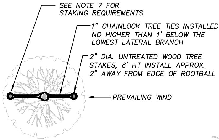
PLAN VIEW STAKING DETAIL
